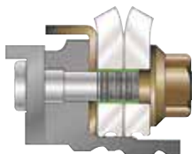
Hub centric nut fills void between stud and hole.
