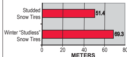
Braking distance on Icy Road - (from 31 mph) Average calculated at different temps
