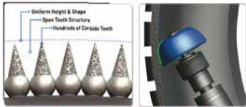
S&S Structured Carbide coatings and unique flared shape maximizes contact, producing a flat, level buffed surface!
