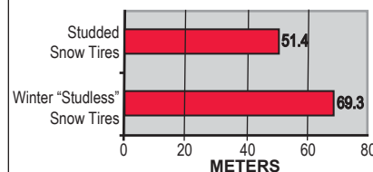
Braking distance on Icy Road - (from 31 mph) Average calculated at different temps
