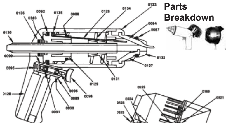
STUD GUN PARTS (AS-9 MODEL)
