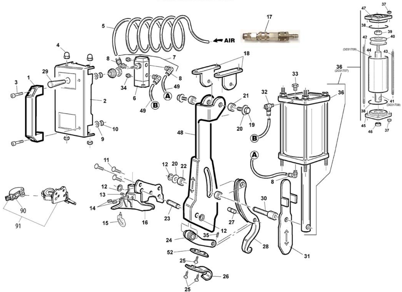
Leverless Bead Lifter
