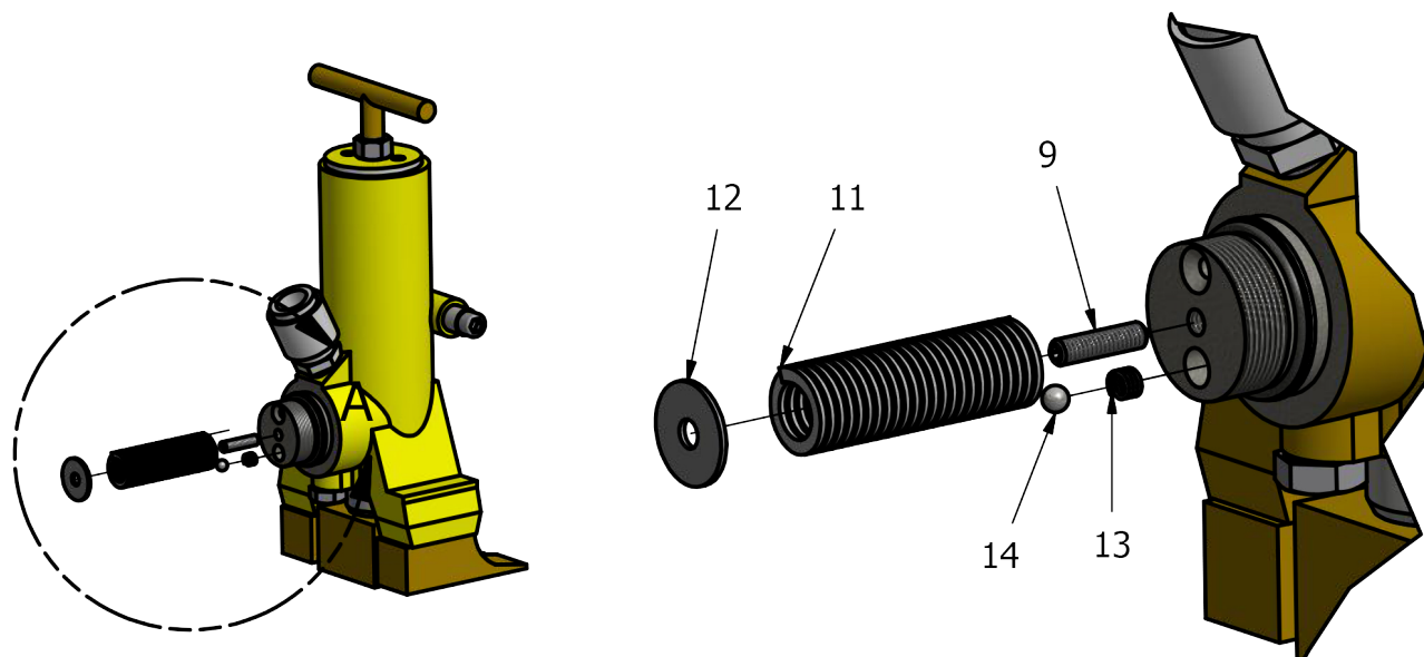
DETAIL A SCALE 1/2
