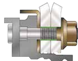
Hub centric nut fills void between stud and hole.
