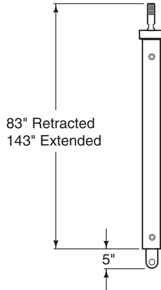
FC5761 Cylinder
