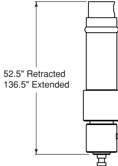
PS130004 Cylinder
