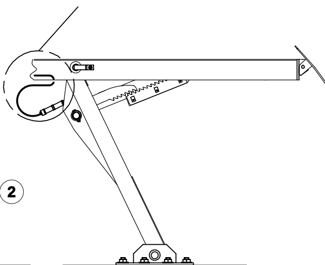
DETAIL B
