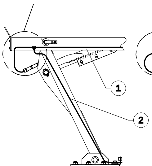
DETAIL A
