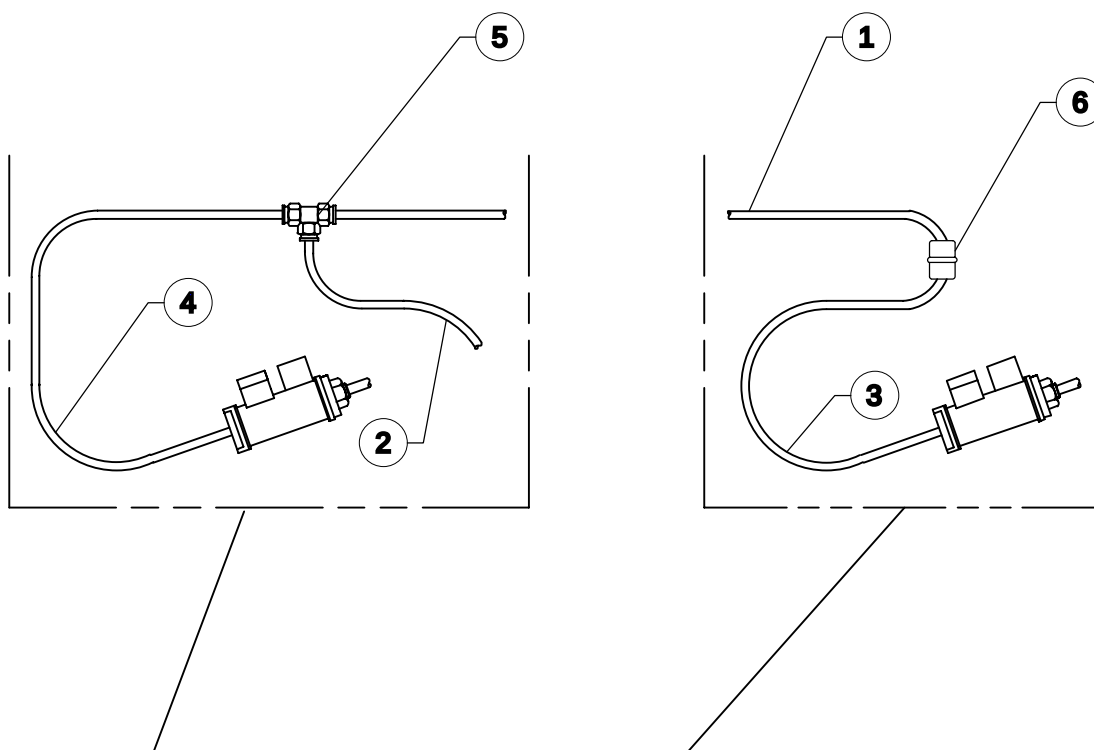
DETAIL A
