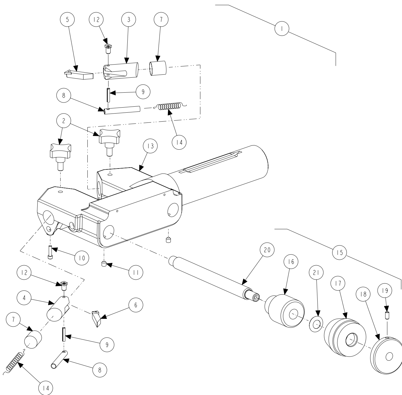
TWIN CUTTER WITHOUT DIGICAL 105-324-1 Only
