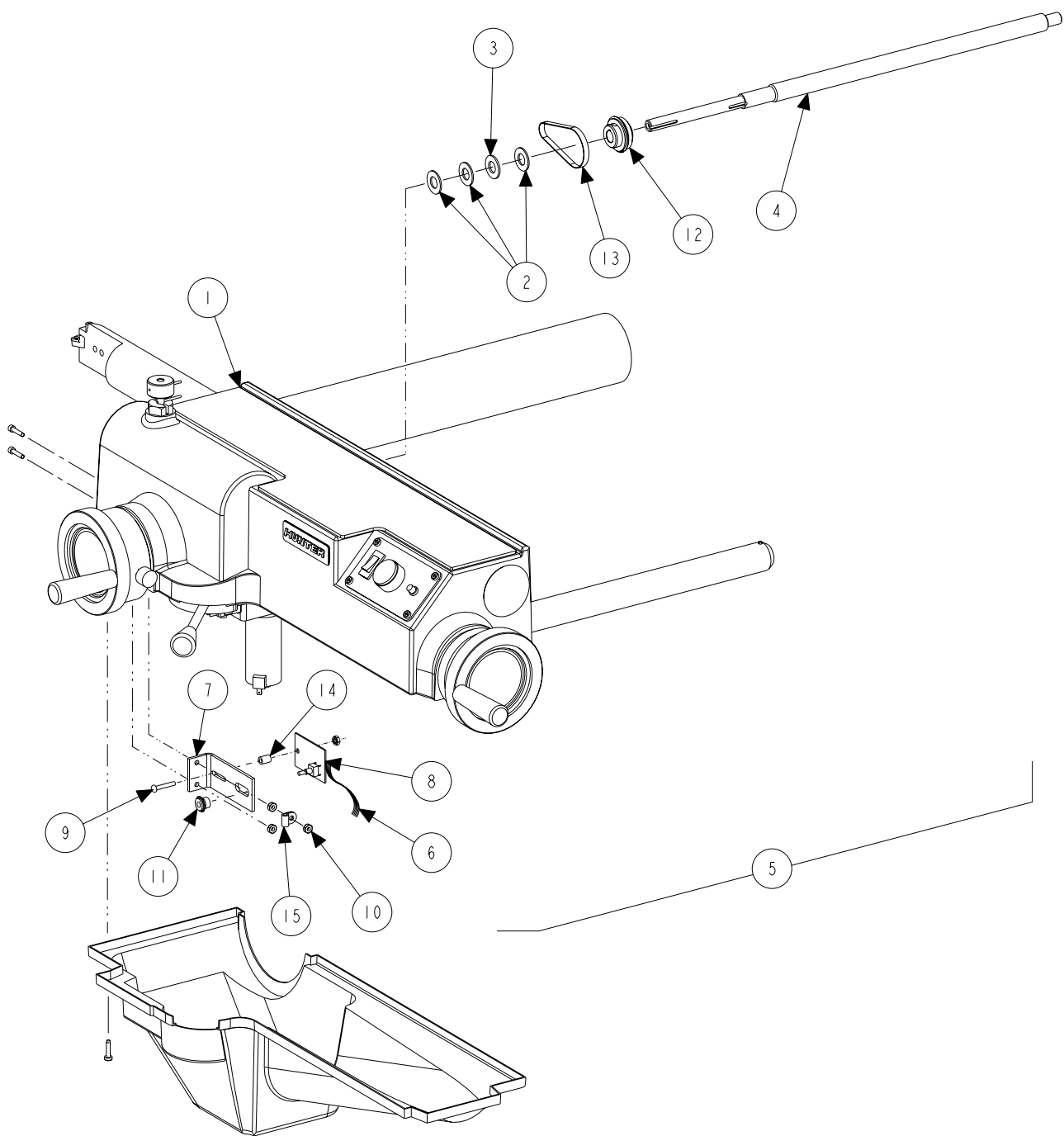
FEED CONTROL HOUSING WITH DIGICAL HOUSING
