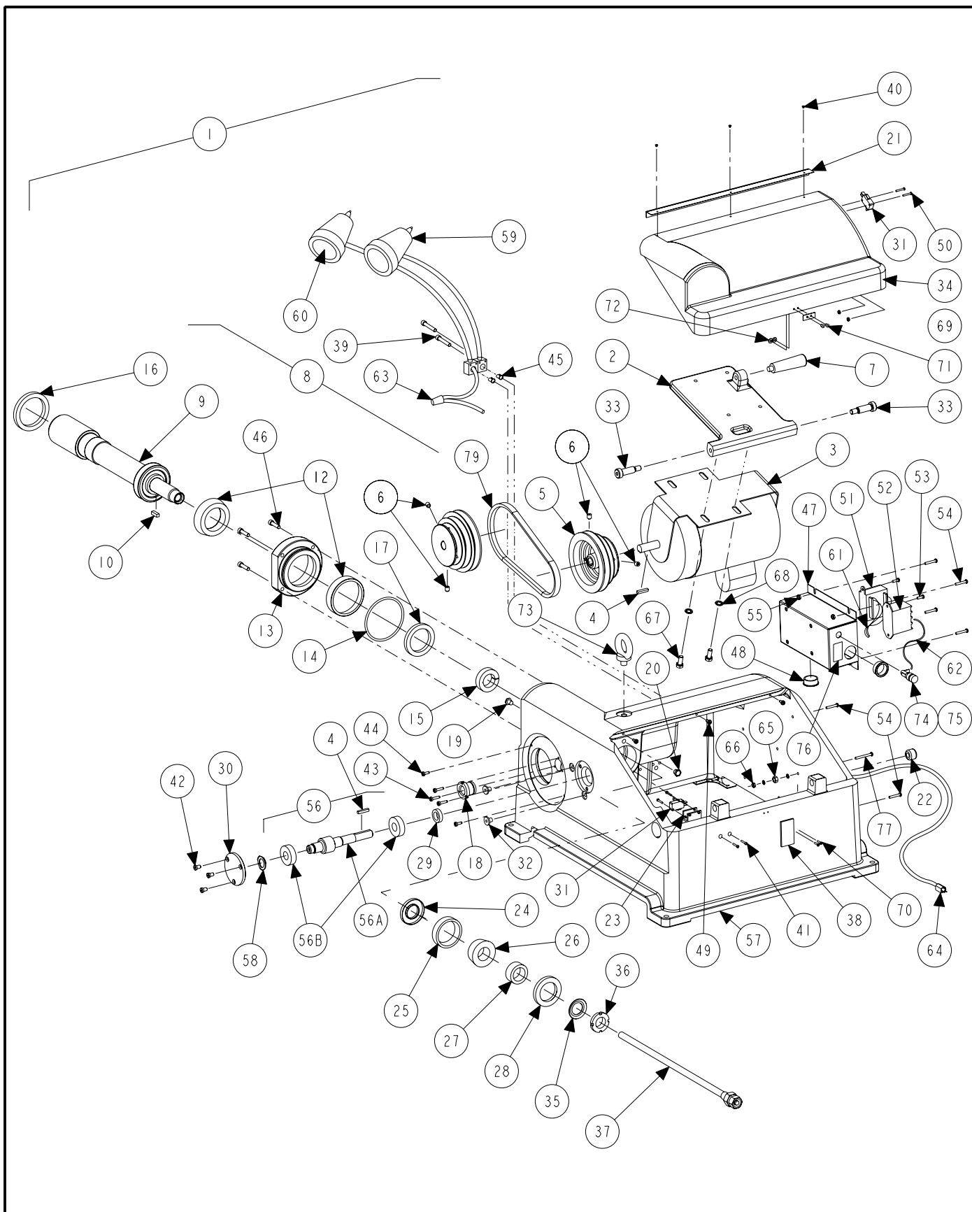
BL500 OFFCAR BRAKE LATHE REFER TO NEXT SHEET FOR PARTS DESCRIPTION LISTING
