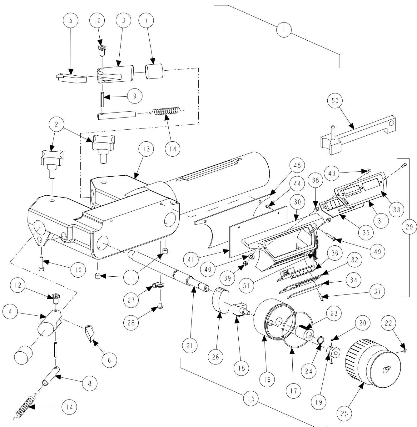
TWIN CUTTER WITH DIGICAL HOUSING 105-325-1 ONLY
