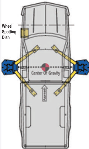
Vehicle Center of Gravity
