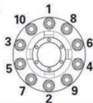
75520 65# torque limiting extension
